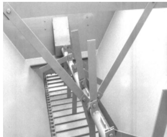
Low rpm flail agitator breaks up bridging in the stickiest materials.
